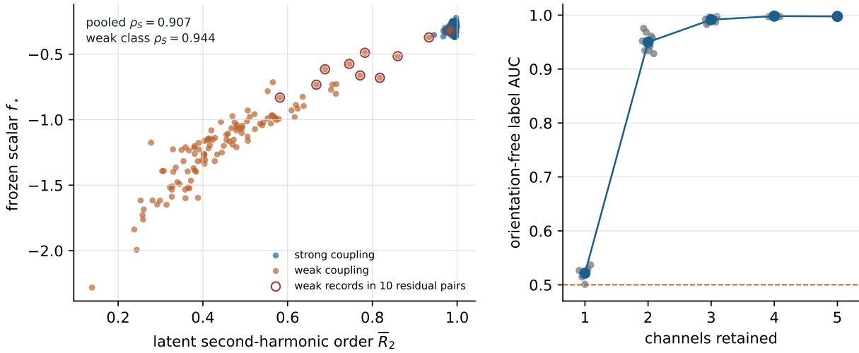
Figure 3: Post-hoc interpretation of the frozen Kuramoto winner. Left: the source-selected scalar tracks latent second-harmonic coherence \bar{R}_2 ; rings mark the weak-coupling records in the ten residual released-match collisions. Right: every point is one of the \binom{5}{m} channel subsets, with canonicalization and both primitives recomputed for that subset; blue points are subset-count means. These are descriptive diagnostics on a result already seen, not a new held-out test.
